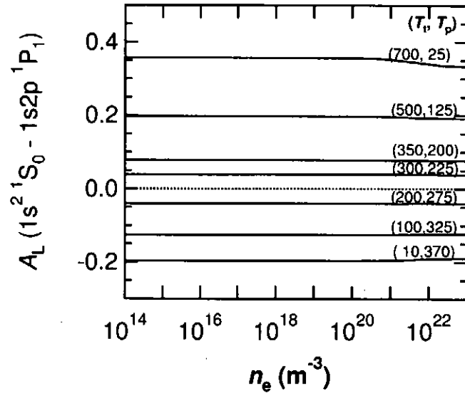
FIG. 79: Calculated longitudinal alignment, A_L , for the emission (1)-(7) 1s^2 1S_0 \leftarrow 1s2p 1P_1 . Two temperature parameters EVDFs are assumed. T_i and T_p , are selected to indicate the same mean squared value of v ; \frac{1}{2}m\langle v^2 \rangle = 250 eV.
