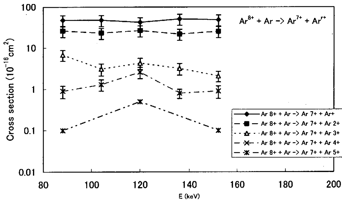
Figure 14. Energy dependence of cross section for \text{Ar}^{8+} + \text{Ar} \rightarrow \text{Ar}^{7+} + \text{Ar}^{r+} processes.
