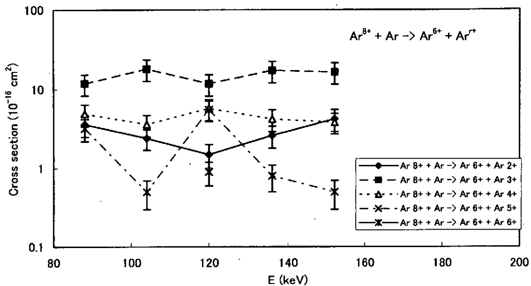
Figure 13. Energy dependence of cross section for \text{Ar}^{8+} + \text{Ar} \rightarrow \text{Ar}^{6+} + \text{Ar}^{r+} processes.
