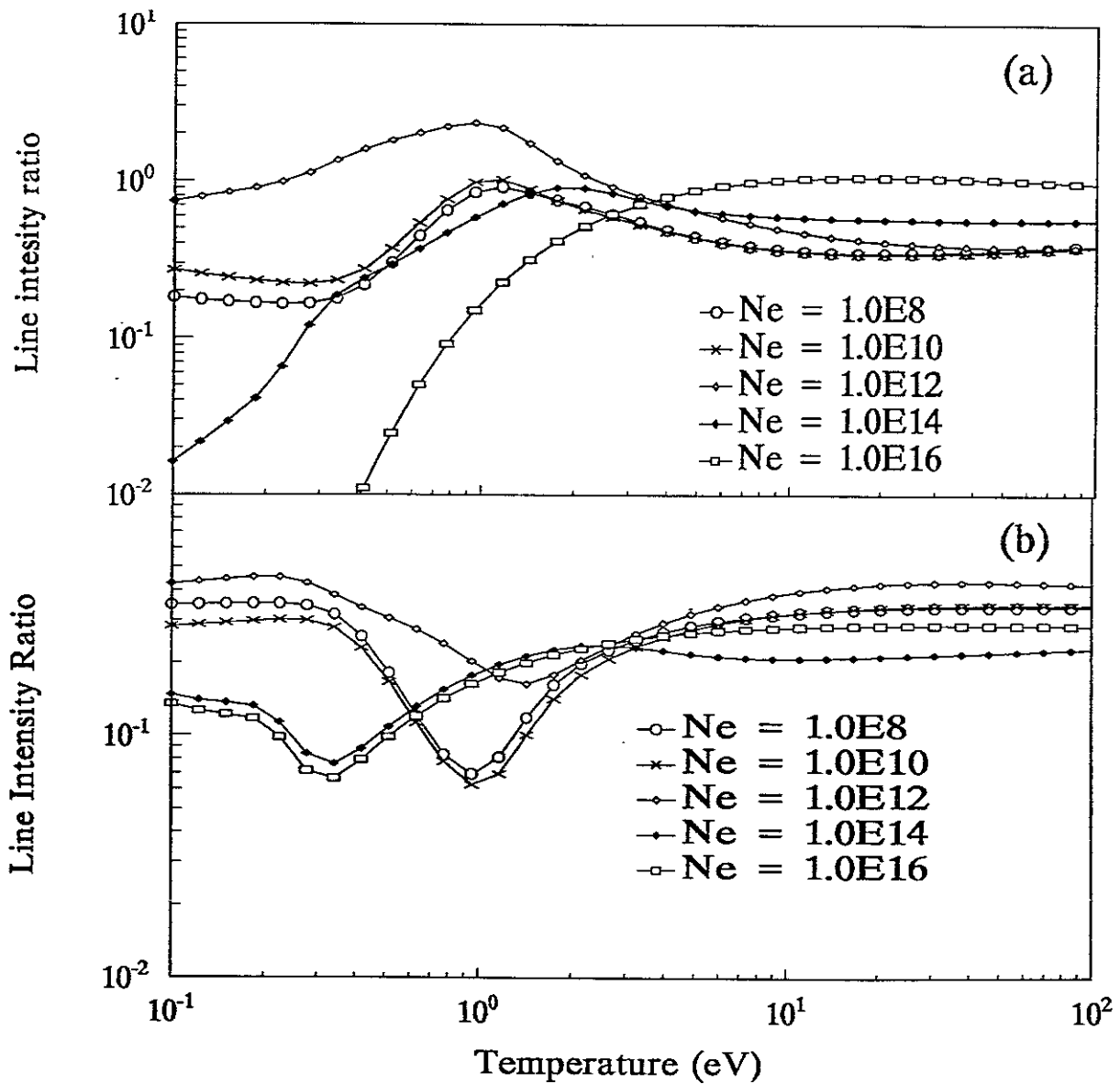
Fig.23 Line intensity ratio as a function of the electron temperature in the recombining plasma. (a). 126 \text{ nm} (2p3d(^3P) \rightarrow 2p2(^3P)) / 193 \text{ nm} (2p3s(^1P) \rightarrow 2p2(^1D)) (b). 160 \text{ nm} (2p4d(^1P) \rightarrow 2p2(^1S)) / 126 \text{ nm} (2p3d(^3P) \rightarrow 2p2(^3P))
