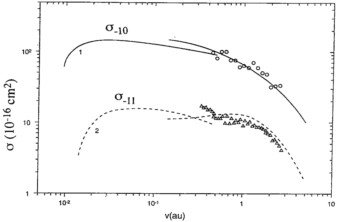
Fig.3. Single- and double-electron detachment cross sections in collisions of two \text{H}^- ions versus velocity of the relative motion. Curves (1) and (2) are calculations [5]. The middle-energy experimental data and theoretical curves are taken from Ref.[14].
