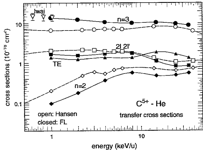
FIG. 17: Calculated electron cross sections in \text{C}^{5+} -He collisions, from close-coupling calculations with AO expansions [33] (closed symbols) and [22] (open symbols), for single electron transfer to n=2,3 states, for double electron transfer to 2l2l' states, and for transfer-excitation (TE) configurations. Data is by Iwai et al. [34] (inverted triangles).
