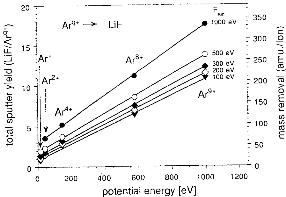
Fig. 25b: Total sputter yields for \text{Ar}^{q+} bombardment of polycrystalline LiF vs. MCI potential energy, for different impact energies [22, 44].
