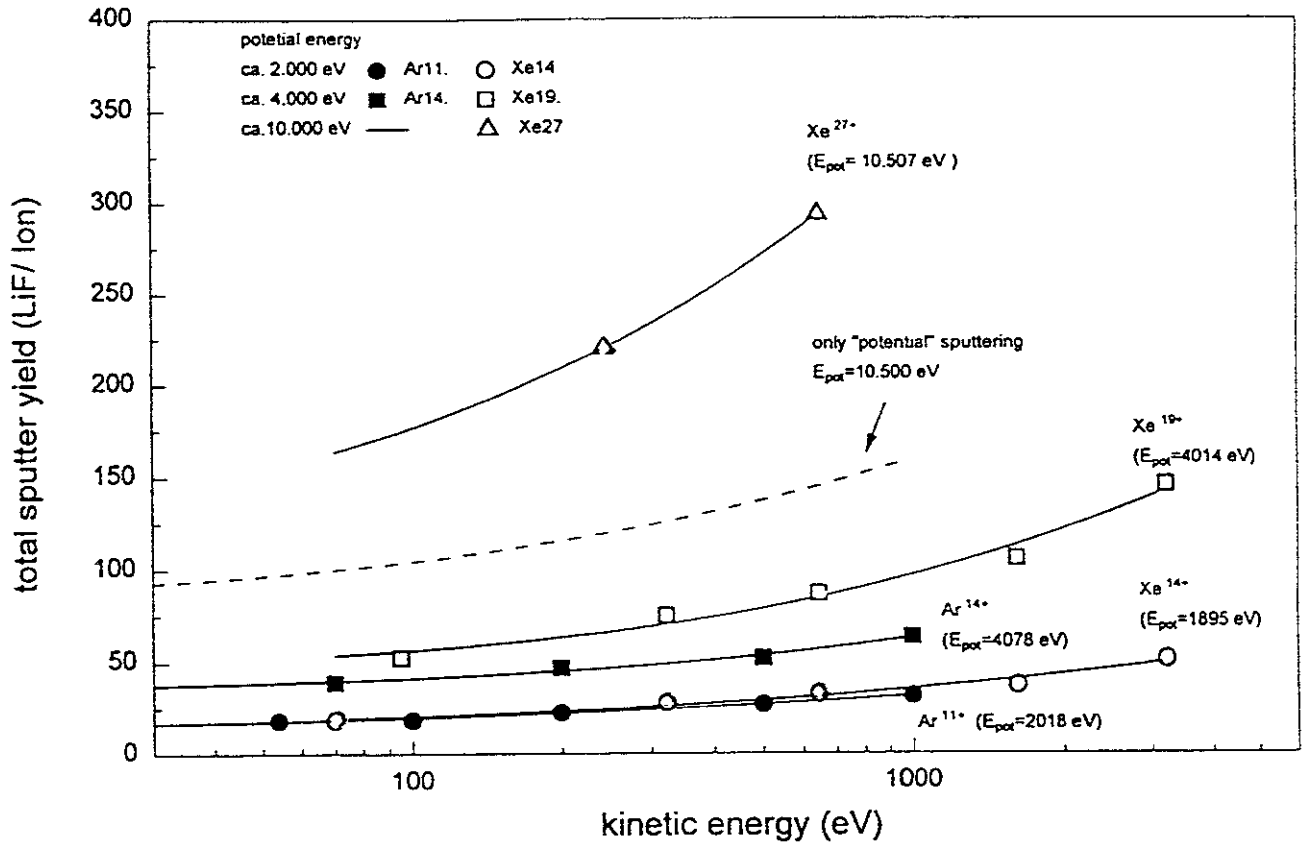
Fig. 26: Total sputtering yields for impact of \text{Ar}^{q+} ( q = 11, 14 ) and \text{Xe}^{q+} ( q = 14, 19, 27 ) on polycrystalline LiF (cf. text).
