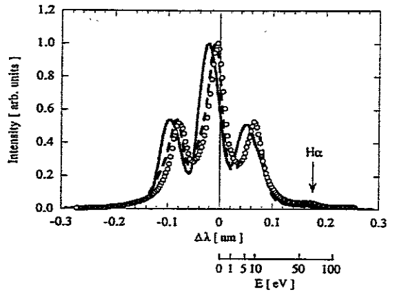
fig. 2 Open circles show measured D\alpha spectrum. Solid and dashed lines show calculated D\alpha spectrum. In the calculation shown by dashed line, Franck-Condon energy was modified.
