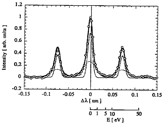
fig. 3 Open circles show measured He I spectrum. Solid thick line shows fitted curve using two Gaussian functions. Thin and dashed lines show the contribution of two Gaussian functions.
