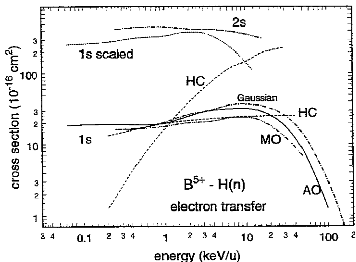
FIG. 5: Calculated total transfer cross sections in collisions between B^{5+} ions and H ( 1s ) and H ( 2s ) targets, from close-coupling calculations with an AO expansion (full line) [11], with a Gaussian expansion [9] (dash-dotted line), with an MO expansion (triple-dot-dashed line) [6], and from the hidden-crossing theory (broken line) [10]. The dotted line is the result of scaling the MO curve for a H ( 1s ) target, for a simple prediction of cross sections from an excited H ( n=2 ) target. The MO curve for the excited H ( 2s ) target indicates the transfer cross section to the n=6-8 states only.
