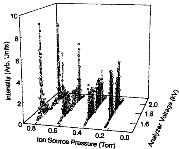
Figure 1.- Energy distribution of H^+ in coincidence with H^- at different ions source pressures.
