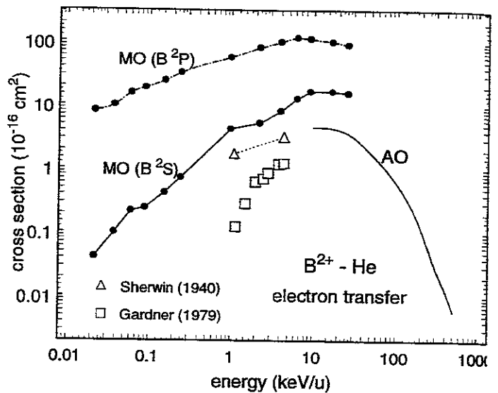
FIG. 16: Calculated electron cross sections for total electron transfer in B^{2+} -He collisions, from MO close-coupling calculations [28] for the B^{2+} \ ^2S ground state (solid line with dots) and the B^{2+} \ ^2P excited state (dash-dotted line), and from a one-electron AO calculation [20] (solid line). Data are by Sherwin [30] (triangles) and by Gardner et al. [29] (boxes).
