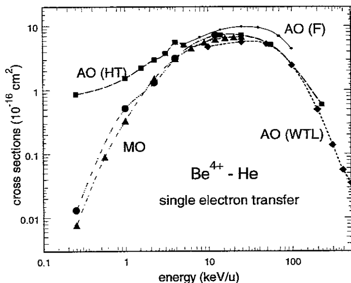
FIG. 8: Calculated single electron transfer cross sections in \text{Be}^{4+} -He collisions, from close-coupling calculations with two-electron AO expansions [19] (full line) and [22] (dashed line with squares), with a one-electron AO expansion [20] (dashed line with diamonds), and with MO expansions [12] (circles) and [23] (triangles).
