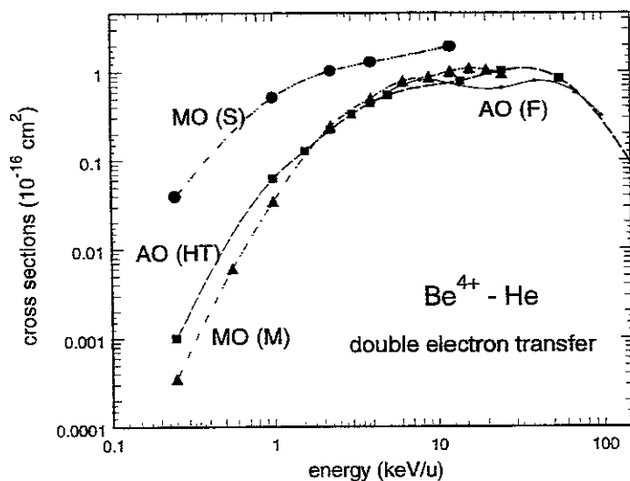
FIG. 9: Calculated double electron transfer cross sections in \text{Be}^{4+} -He collisions, from close-coupling calculations with AO expansions [19] (full line) and [22] (dashed line), and with MO expansions [12] (circles) and [23] (triangles).
