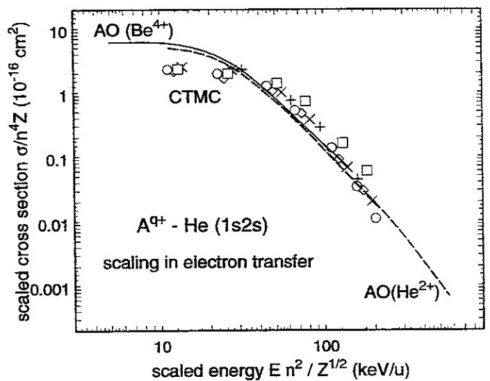
FIG. 13: Scaled plot of calculated electron transfer cross sections in A^{Z+} - \text{He}(2s) collisions, from close-coupling calculations for \text{Be}^{4+} [24] (full line) and \text{He}^{2+} [17] (dashed line) projectiles, and from a CTMC study [25] for \text{Li}^{3+} (+), \text{Be}^{4+} ( \times ), \text{B}^{5+} ( \diamond ), \text{C}^{6+} ( \circ ), and \text{O}^{8+} ( \square ) projectiles.
