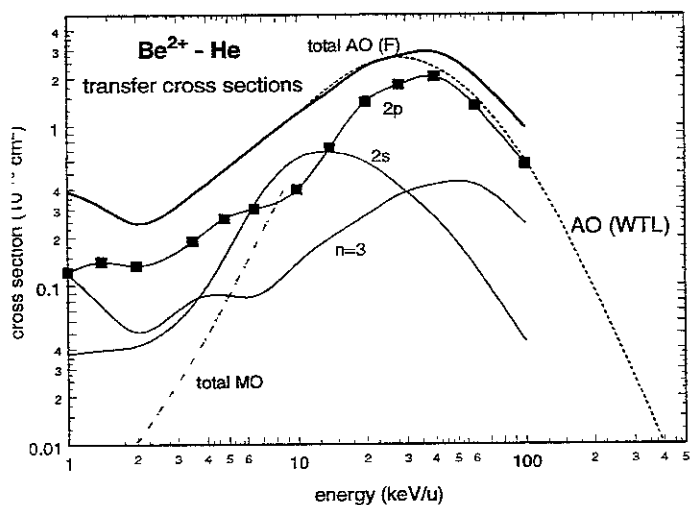
FIG. 7: Calculated total transfer cross sections in \text{Be}^{2+} -He collisions, from close-coupling calculations with a two-electron AO expansion (full line) [21] and with a one-electron AO expansion [20] (dashed line), and with an MO expansion (triple-dot-dashed line) [12]. The other lines are partial single transfer cross sections [21] to projectile states as specified in the figure.
