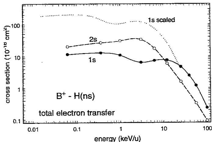
FIG. 4: Calculated total transfer cross sections in collisions between B^+ ions and H ( 1s ) (full line) and H ( 2s ) (broken line) targets, from close-coupling calculations with AO expansions [11]. The dotted line is the result of scaling the full line for a simple prediction of cross sections from an excited H ( n=2 ) target.
