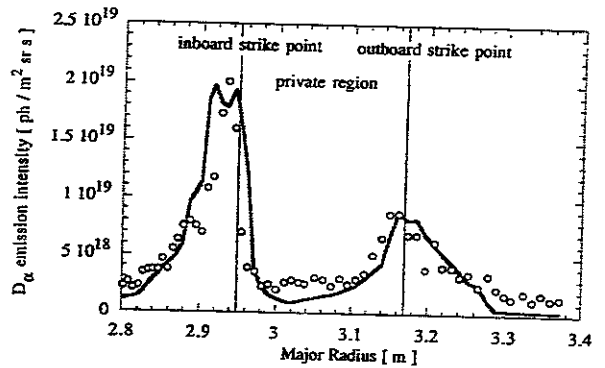
fig. 4 Open circles and solid line show measured and calculated D\alpha emission intensity profile, respectively.
