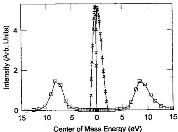
Figure 2.- Center of mass energy distribution of H^+ and H^- from the H_3^+ polar dissociation on He at 8 keV, in the forward and backward directions. The crosses represents the H^- fragment and the squares the H^+ fragment.
