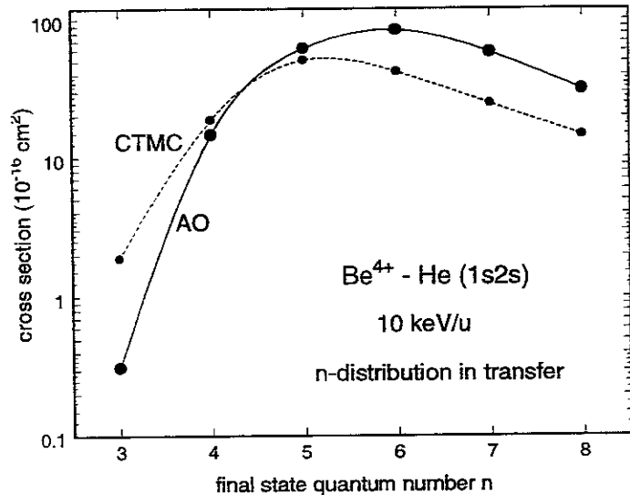
FIG. 12: Calculated n -distribution of electron transfer cross sections in \text{Be}^{4+} - \text{He}(2s) collisions, from close-coupling calculations with a one-electron AO expansion [24] (full line), and from a CTMC study [25] (dashed line).
