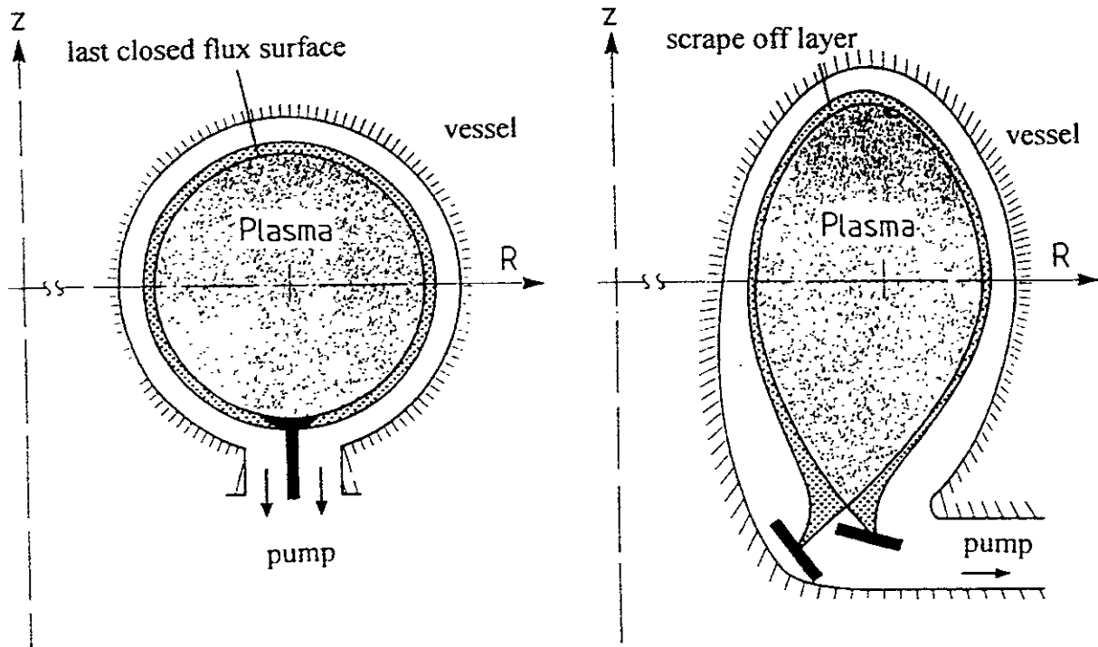
Fig. 1: Schematic of plasma boundary - limiter (left) and divertor (right) /1/.
