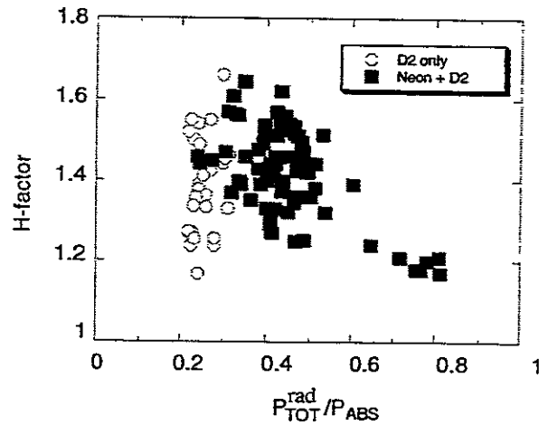
Fig. 3 H-factor vs P_{\text{TOT}}^{\text{rad}}/P_{\text{ABS}} in ELMy H-mode plasmas with neon and deuterium gas puff. ( P_{\text{NB}} < 23\text{MW} )
