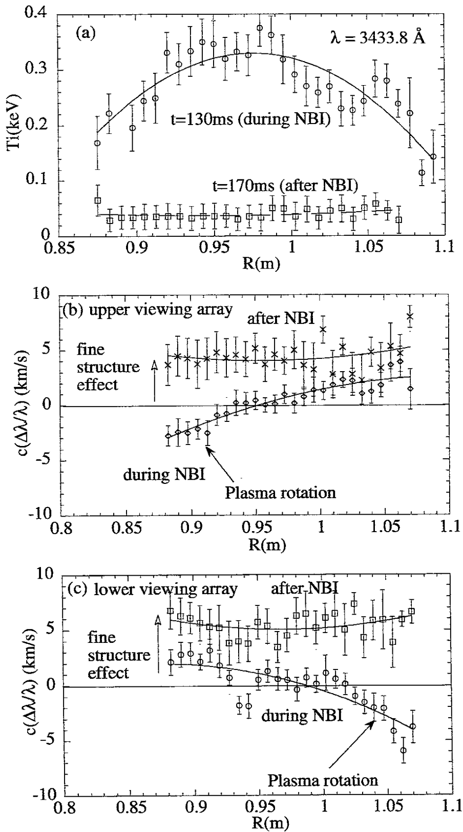
Fig.6 Radial profiles of (a) ion temperature and (b),(c) wavelength shift ( \Delta\lambda ) of \Delta n \cong 7 - 6 transition measured with (b) upper viewing array and (c) lower viewing array during NBI and after NBI was turned off
