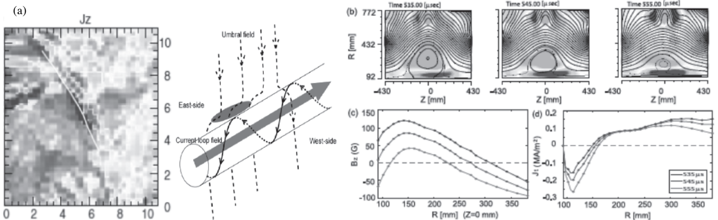
Fig. 1 (a) Light-Bridge phenomenon observed at a sun spot (left) and its most-probable field-line structure (right). (b) Snapshot images of spheromak and OH field. Thick contours show magnetic field lines at regular intervals and thin contours are complementary to emphasize reconnecting field lines. Color bar indicates toroidal current density measured by the 2D magnetic probes. (c) The radial profile of B_z component and (d) the toroidal current J_t on the mid-plane
