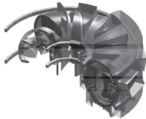
Fig. 1. 3-D design of FFHR-d1.
