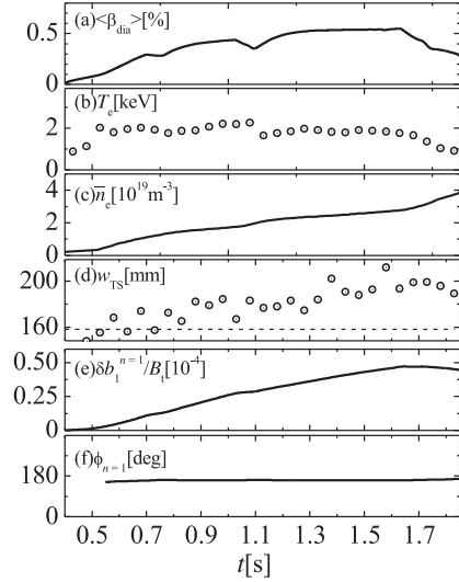
Fig. 3 Time evolution of (a) averaged beta \langle \beta \rangle_{\text{dia}} (b) electron temperature T_e (c) averaged electron density n_e (d) island width w_{\text{TS}} (e) amplitude of n=1 mode \delta b_1 (f) toroidal angle \phi_{n=1}
