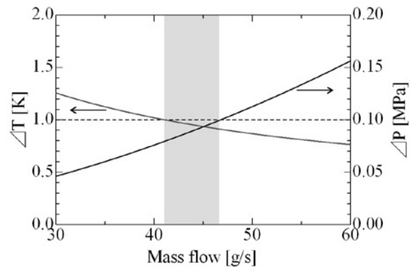
Fig. 2. Temperature rise and pressure drop of SHe between the inlet and the outlet of the CICC when the SHe mass flow through the CICC was changed.
