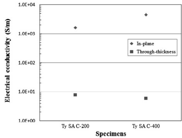
Fig. 2. Electrical conductivities on thickness of carbon interface layer of SiC fiber electrical conductivity of NITE-SiC/SiC composites was investigated. Uni-directional (UD) SiC fibers were used for fiber reinforcement. The SiC fibers used were Tyranno SA fibers with a carbon coating by CVD method. Two specimens with different carbon coating thickness were used. The thickness was 200nm (Ty SA C-200) or 400nm (Ty SA C-400), respectively. The NITE-SiC/SiC composites were sintered by Hot Press at 1850°C with 20MPa sintering pressure.
