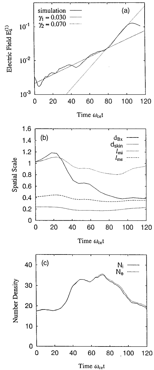
FIG. 2. Temporal evolutions of (a) the reconnection electric field E_z^{(1)} , (b) four spatial scales, and (c) the electron number density (dotted line) and the ion number density (solid line) at the reconnection point for the same case as Fig. 1. Here d_{Bx} , d_{skin}=c/\omega_{pe} , l_{mi} and l_{me} in (b) are the scale height of magnetic field B_x , the electron skin depth, the average orbit amplitude of meandering ions and that of meandering electrons, respectively.
