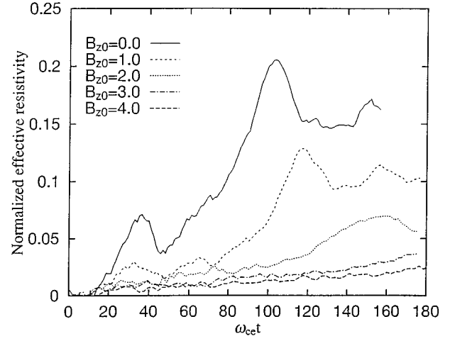
FIG. 14. Temporal evolution of the effective resistivity for five different values of B_{z0} where the resistivity is normalized by the Hall resistivity B_0/qcn_e .
