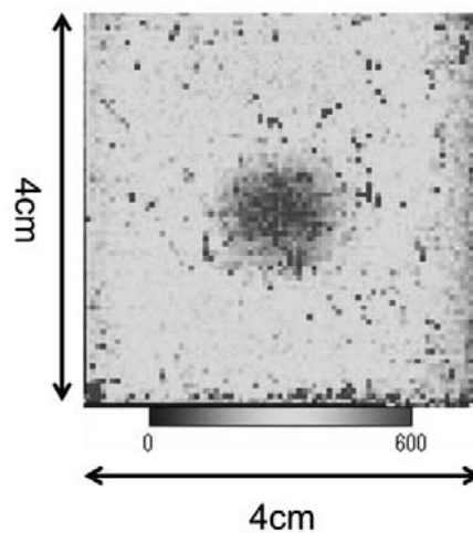
Fig. 2 Track density in the emulsion for shot #8963-#8969 of KSTAR deuterium plasma.
