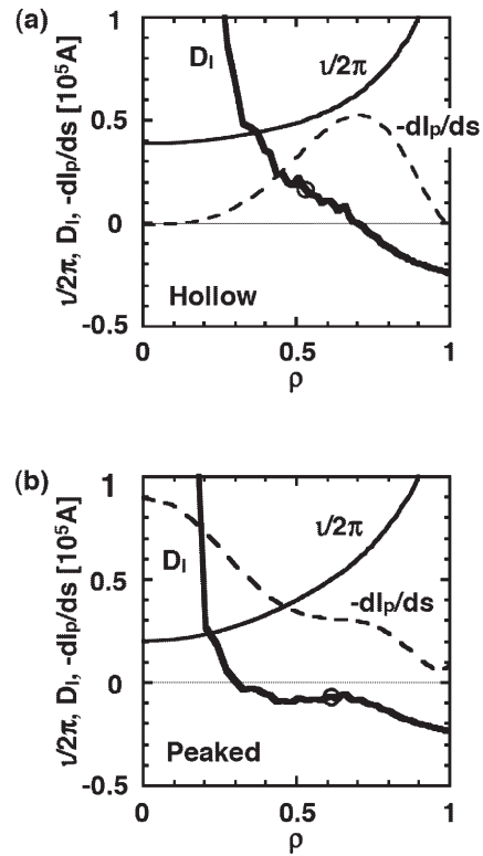
Fig. 1. Profiles of rotational transform ( \nu/2\pi ), the Mercier parameter ( D_1 ) and current density ( -dI_p/ds ) for different current profiles: (a) hollow current profile and (b) peaked current profile. In each figure, the location of \nu/2\pi=0.5 is indicated on the D_1 profile with an open circle.
