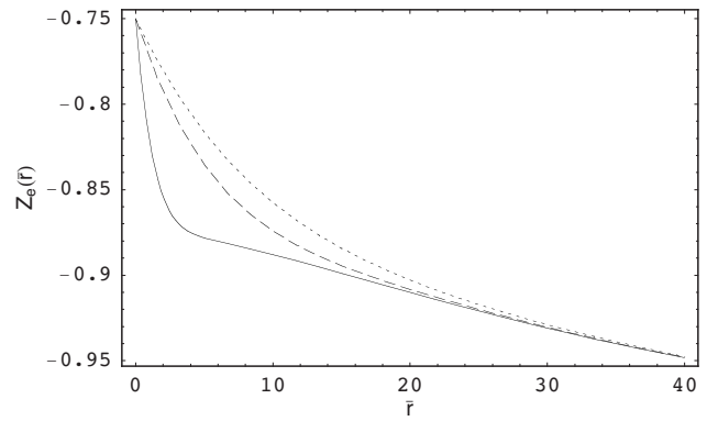
FIG. 2. The renormalized electron charge Z_e as a function of the scaled distance \bar{r} when Z=2 and \bar{r}_D=30 . The solid line represents the case of \bar{\lambda} = 1 . The dashed line represents the case of \bar{\lambda}=4 . The dotted line represents the case of \bar{\lambda}=6 .
