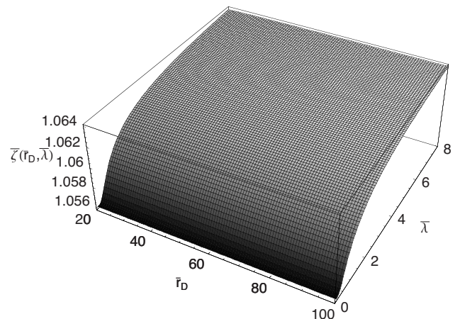
FIG. 3. The three-dimensional plot of the Wannier exponent \bar{\zeta} as a function of the scaled Debye length \bar{r}_D and scaled de Broglie wavelength \bar{\lambda} when Z=2 .
