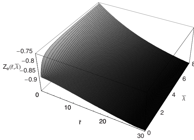
FIG. 1. The three-dimensional plot of the renormalized electron charge Z_e as a function of the scaled de Broglie wavelength \bar{\lambda} and scaled distance \bar{r} when Z=2 and \bar{r}_D=20 .
