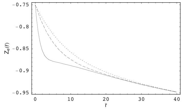
FIG. 2. The renormalized electron charge Z_e as a function of the scaled distance \bar{r} when Z=2 and \bar{r}_D=30 . The solid line represents the case of \bar{\lambda}=1 . The dashed line represents the case of \bar{\lambda}=4 . The dotted line represents the case of \bar{\lambda}=6 .
