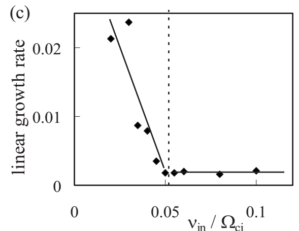
FIG. 12. (a) Density profiles at the saturation phase with v_{in} = 0.02, 0.04, 0.05, 0.08, 0.1 . The densities are normalized by those at r=0 . The dashed line shows the solution of the linearized equation of Eq. (1), which corresponds to the case without the convective nonlinearity. (b) Dependencies of the instantaneous linear growth rate calculated with density profiles in (a) on the azimuthal mode number, and (c) that of (4, 1) mode on v_{in} .
