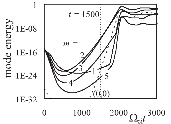
FIG. 1. Time evolution of the potential energy of each Fourier mode in the case with \nu_{in}=0.1 .
