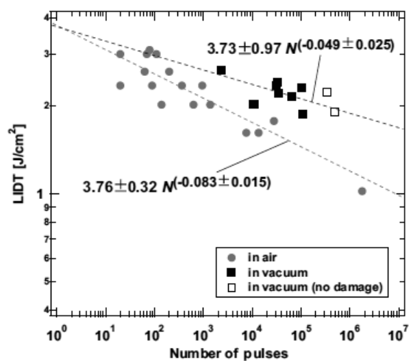
Fig. 2 Multi-pulse LIDT for OFHC Cu mirrors in air atmosphere and vacuum condition.
