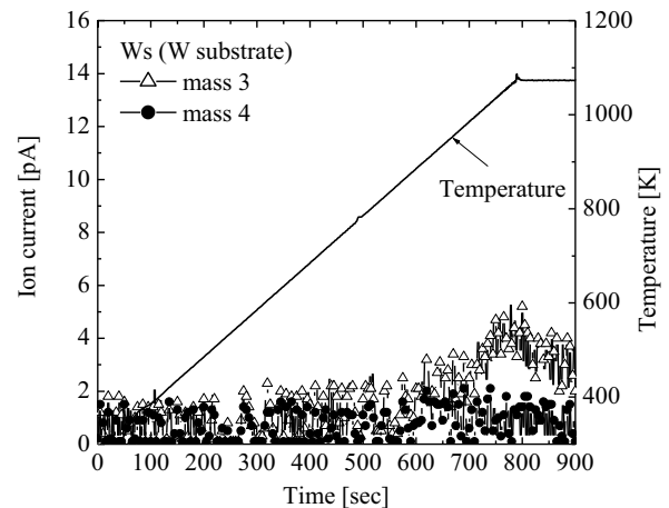
Fig.3 Deuterium release behavior from sample Ws.
