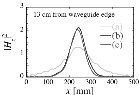
Fig. 2. Profiles of the wave field power for the three cases of Fig. 1.
