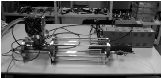
Fig. 1. Experimental setup.
