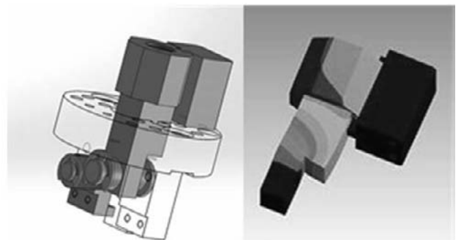
(a) The configuration of tensile mechanism (b) The ANSYS stress analysis of applied uniaxial tensile strain mechanism
