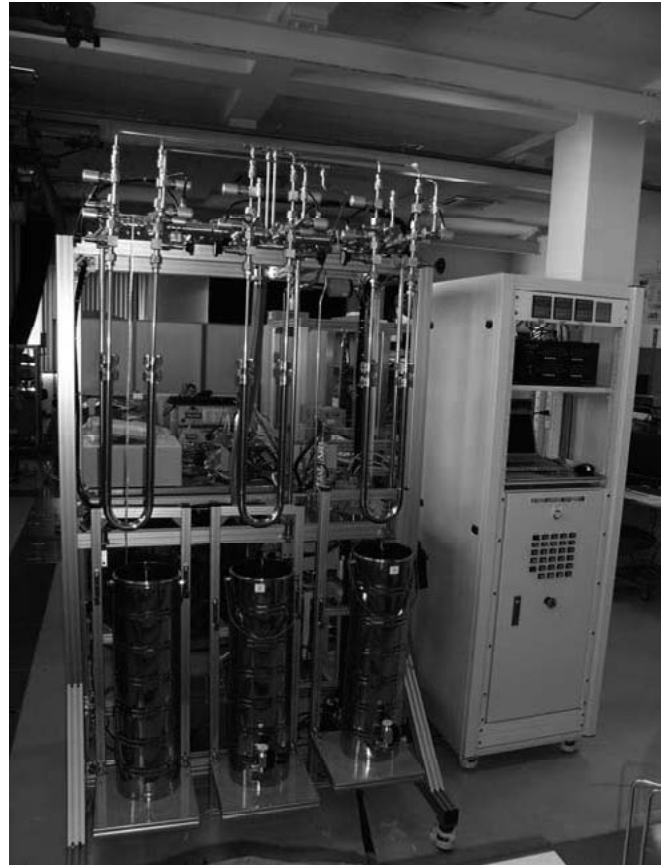
Fig. 1 Snapshot of the newly made apparatus of a pressure swing cryogenic adsorption process system with three packed-columns for hydrogen isotope separation.
