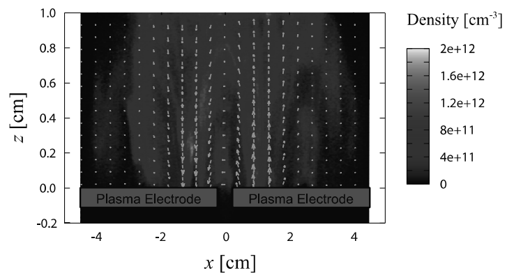
Fig.2 Magnetic field represented with vector field and a contour plot of electron density in x-z plane
