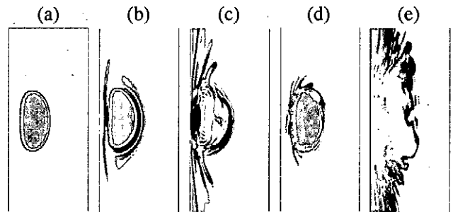
Fig. 2. Nonlinear time development of pressure profile. (a)t=0( \tau A ), (b)500, (c)620(n=1), (d)60, (e)320(n=6).
