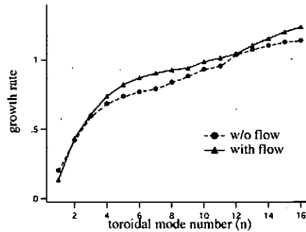
Fig. 1. Linear growth rate of the instabilities for each toroidal mode numbers(n).
