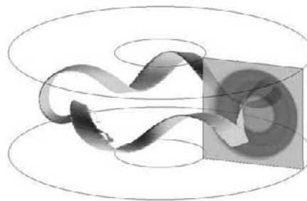
Fig. 1: A relaxed helical structure for the tearing-mode evolution in the RFP.
