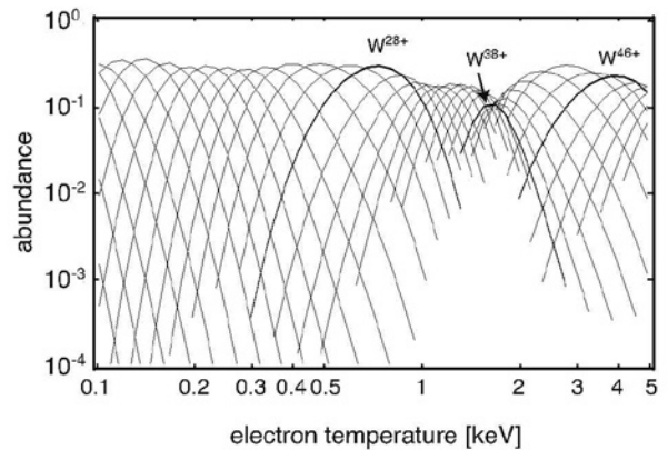
Fig. 1 Ion abundance distribution of W ions in ionization equilibrium calculated by the first CR model in which only configurations are considered 2) .
