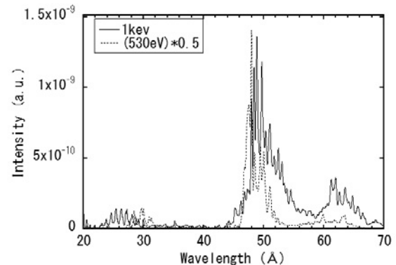
Fig. 2. Synthesized extreme ultraviolet spectra calculated with the second CR model in which fine structure levels are considered for each ion. Electron temperature of 1\text{keV} (solid line) and 530\text{eV} (dashed line) are assumed. Ion abundances are calculated with the first CR model.
