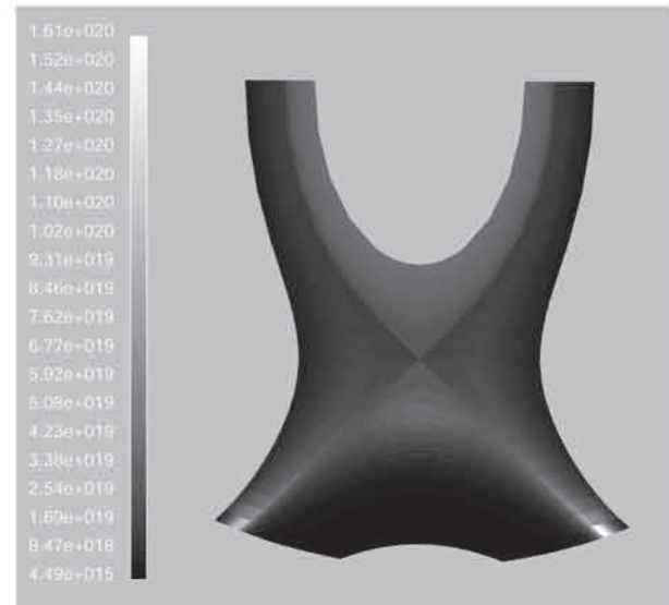
Figure Ion density n_i profile
