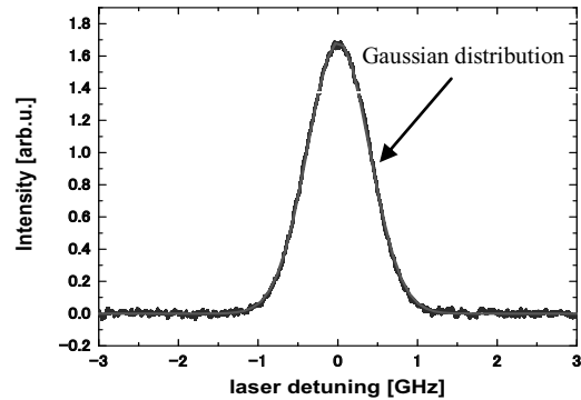
Fig.2. LIF spectrum for argon neutral particles.
