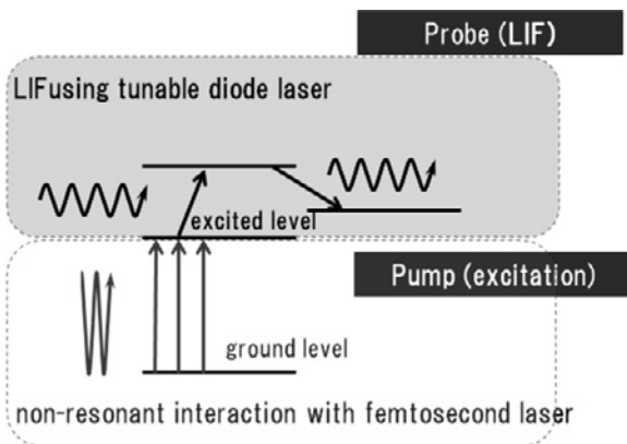
Fig.1 Two-step excitation diagram of LIF system with femtosecond laser.
