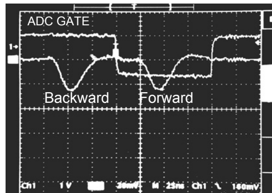
Fig.2. Waveform of the backward and forward scattering signals detected by a wavelength channel in a polychromator. Upper square wave is the gate pulse for analog-to-digital converters.
