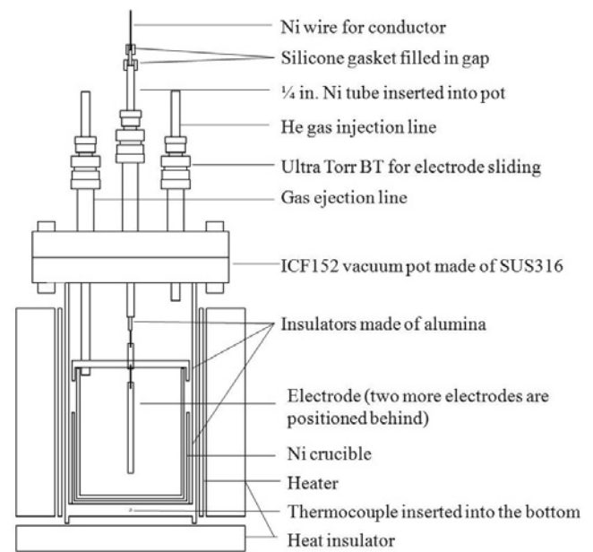
Fig. 1 CAD image of experimental system
