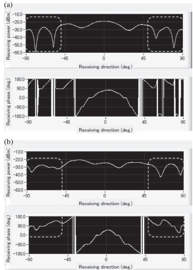
Fig. 1. Test measurements of the diffraction CT subsystem with 10GHz plane wave: (a) for a metal pillar phantom, (b) for an acrylic pillar phantom.
