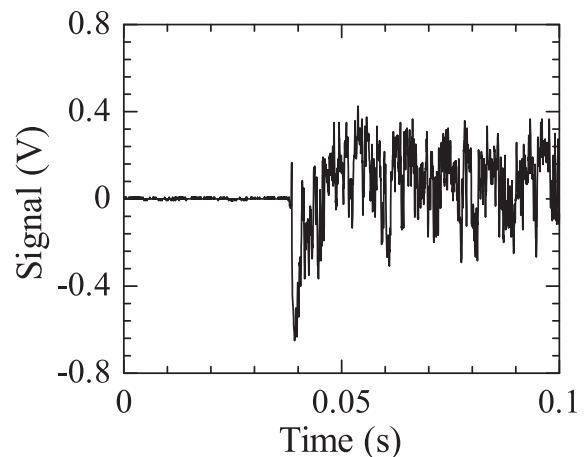
Fig. 2. Waveform of induced voltage of piezoelectric transducer as a function of time.
