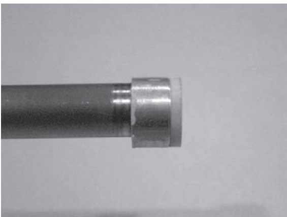
Fig. 1. Piezoelectric transducer with a cylindrical support.
