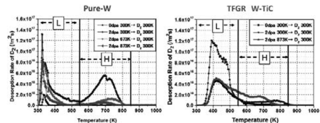
Fig. 4 Effects of higher temperature irradiation on desorption of D 2 for pure W and TFGR W-1.1TiC
