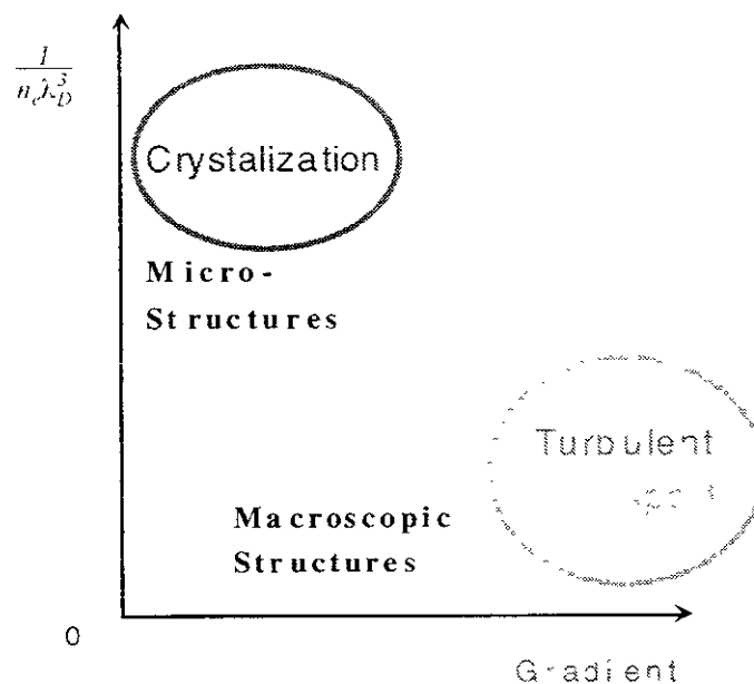
Fig.2 Direction of research on structures in plasmas
