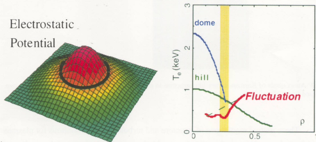
Fig.5 Potential structure, plasma temperature and fluctuations. (Quoted from [3].)
