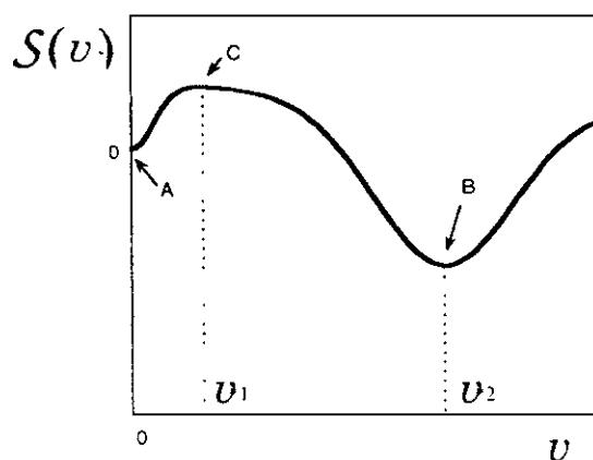
Fig.8 Renormalized dissipation function as a function of the fluctuation level. (Schematic, quoted from [7].)
