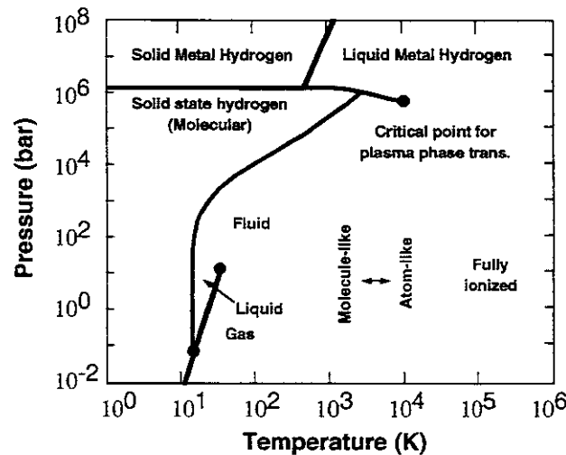
Fig.11 Phase diagram of the hydrogen (Quoted from [10])
