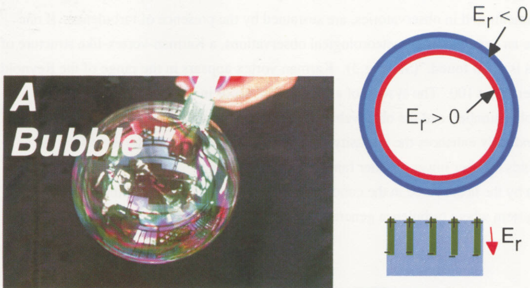
Fig.4 Radial electric field in a bubble. Bubble (a) and schematic drawing of the radial electric field (b). Polymers are aligned normal to the surface. One end of the polymer is positively ionized: this end is much more solvable to oils, not to water. The other end the polymer is negatively charged: this end is akin to water. Electric field normal to the surface is generated near the surface.
