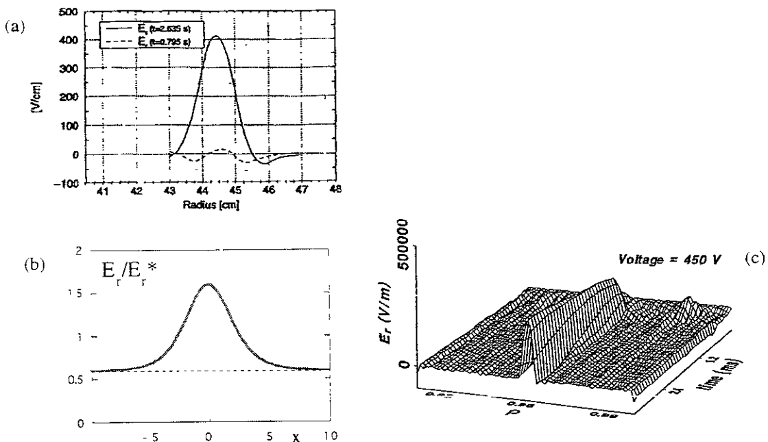
Fig.13 Bifurcation to solitary radial electric field near plasma edge induced by the biased limiter. Experimental result (a) [18], theory (b) [19] and Monte Carlo simulation (c) [20].
