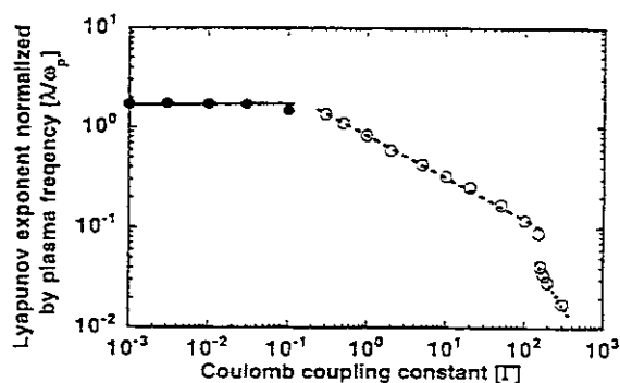
Fig.9 Lyapunov exponents of electron motion in homogeneous plasmas. (Quoted from [8].)
