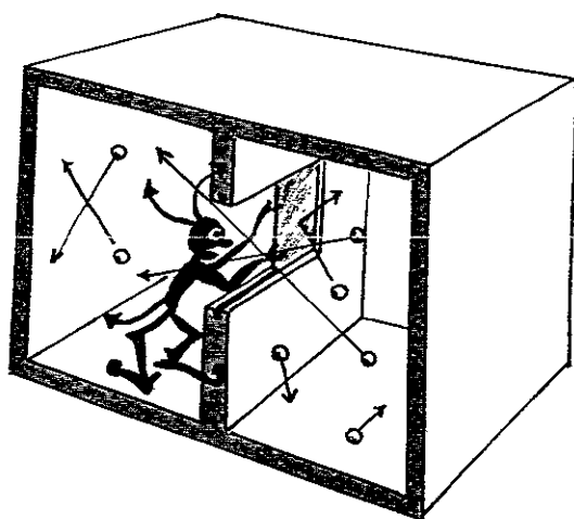
Fig.10 Maxwell's demon (reproduced from [9]).
