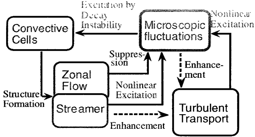
Fig.7 Mutual regulations of microscopic fluctuations and mesoscale structures.
