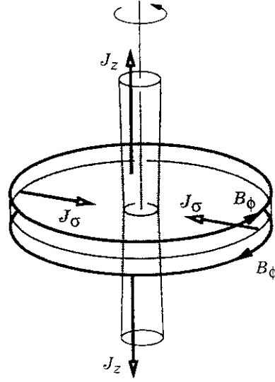
Fig.12 A model of accretion disk (quoted from [4]).
