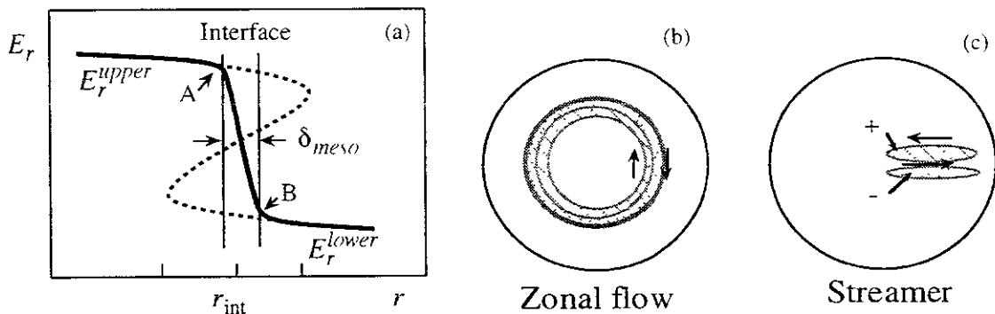
Fig.6 Radial structure of the electric field domain interface (a). Zonal flow (b) and streamer (c) are illustrated on the poloidal cross-section.
